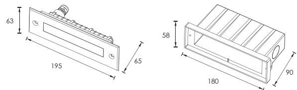
Mounting sleeve
